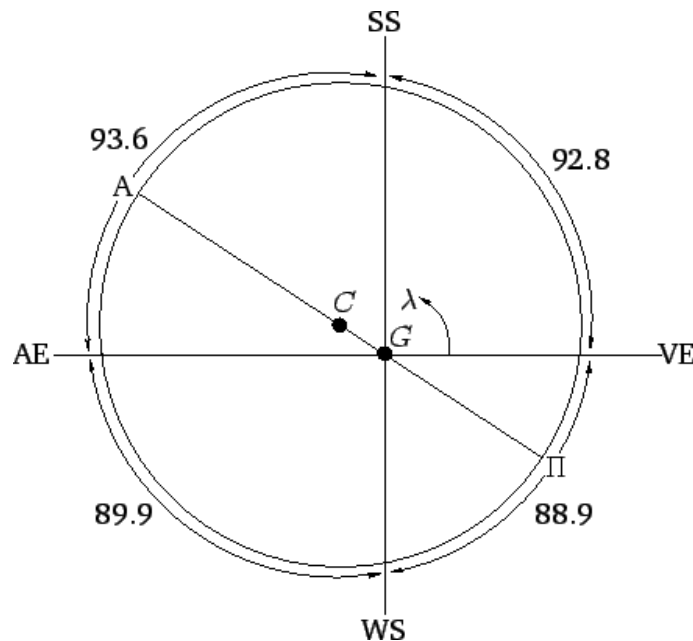
Figure 1: The sun's apparent orbit around the earth, G , showing the vernal equinox (VE), summer solstice (SS), autumnal equinox (AE), and winter solstice (WS). Here, \lambda , \Pi , A , and C are the ecliptic longitude, perigee, apogee, and geometric
